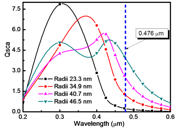
FIG. 2. Scattering cross sections of Ag nanoparticles with different particle diameters.
