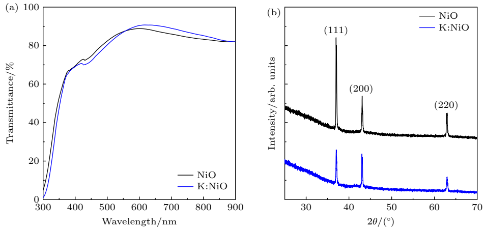
图 3 K + 掺杂前后 NiO 的光学及晶体结构变化,即玻璃上 NiO 和 3% K + 掺杂 NiO 薄膜的 (a) 透射率和 (b) GIXRD 图谱 Fig. 3. Changes in optical and crystal structure of NiO films before and after K + doping: (a) Transmittance and (b) GIXRD of NiO and 3% K + -doped NiO films deposited on glass.
